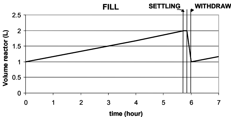
Figure 2.3. Schematic presentation of a six-hour SBR cycle.
