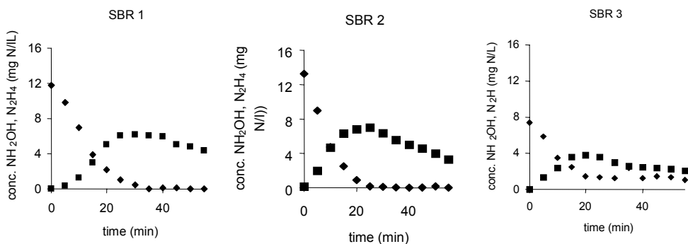
Figure 4.9. Results of hydroxylamine tests in SBR1, 2, and 3 (◆ = NH 2 OH, ■ = N 2 H 4 ).
