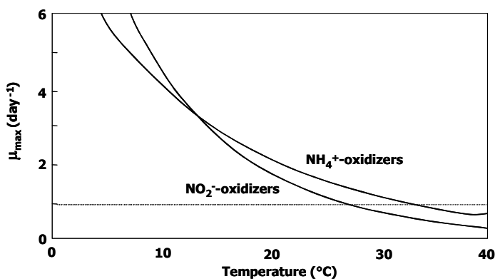
Figure 2.1. The effect of temperature on the maximal growth rate of ammonium and nitrite oxidisers (Hunik 1993). At higher temperatures impaired with a short retention time, nitrite oxidisers can be selectively washed out from the system.
