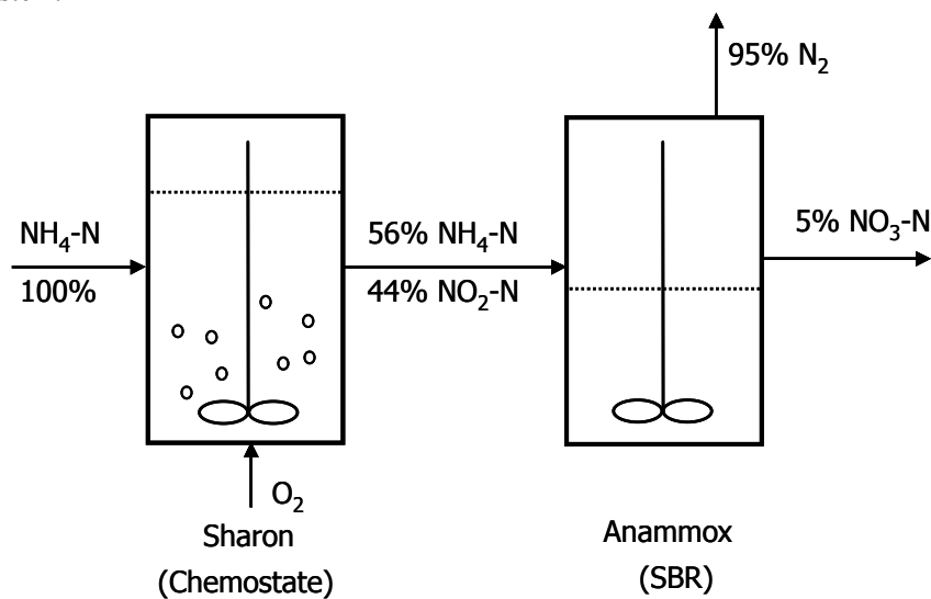
Figure 2.4. Schematic presentation of the combined Sharon/Anammox system.
