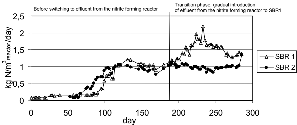
Figure 4.6. Anammox activity in SBR1 (without Anammox inoculum) and SBR2 (with Anammox inoculum).
