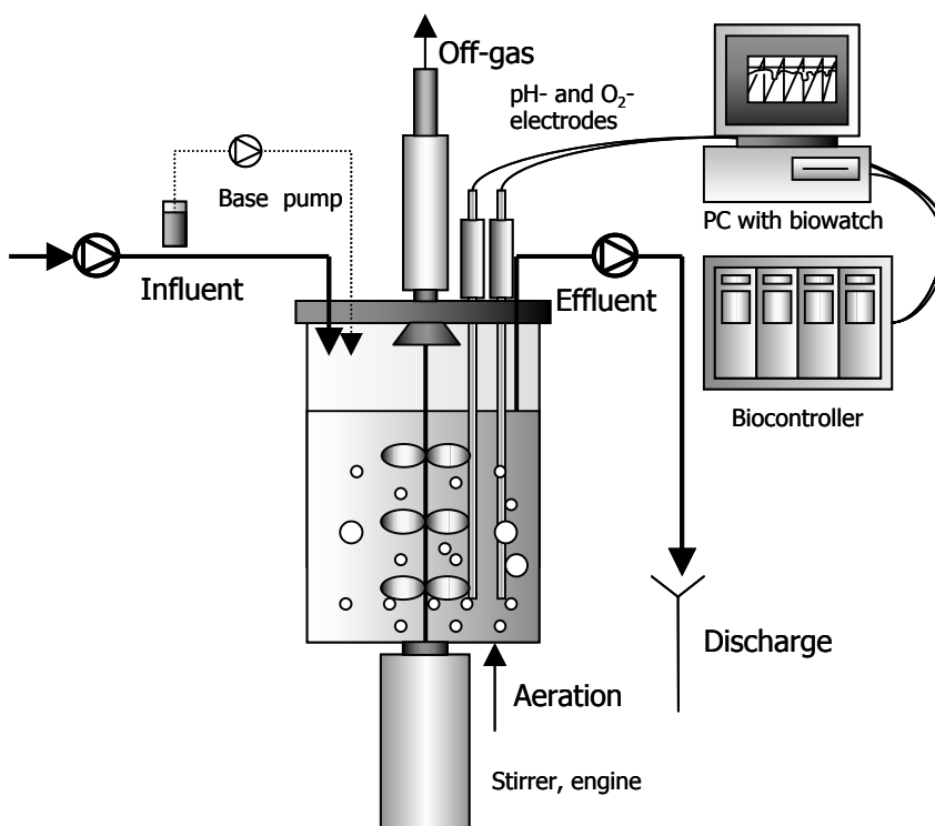
Figure 3.1. Schematic presentation of the Sharon reactor.
