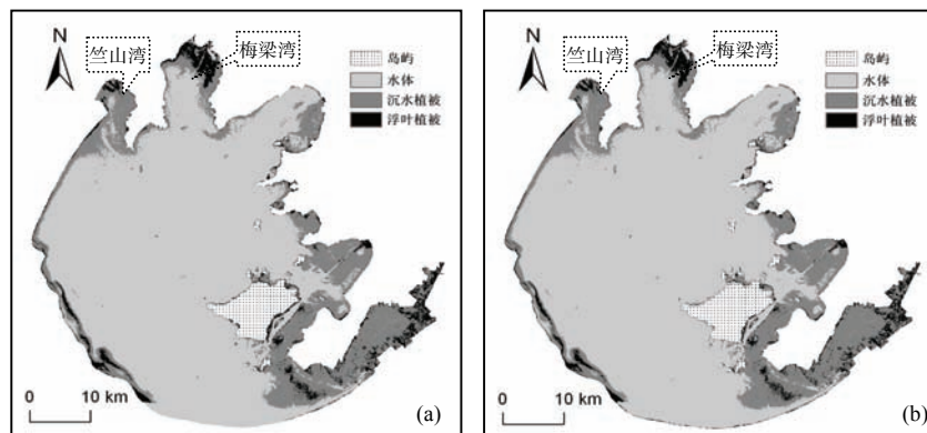
图 5 无透明度参与的太湖水生植被分类(水体、以沉水植被为主导的水生植被类、以浮叶植被为主导的水生植被类): (a)利用 RVI 的分类结果; (b)利用 NDVI 分类结果 Fig.5 Hydrophytes classification result (including water body, submerged vegetation-dominated hydrophytes and floating vegetation-dominated hydrophytes), using the following vegetation index only based on the image pixel statistical feature: (a) RVI vegetation index; (b) NDVI vegetation index
