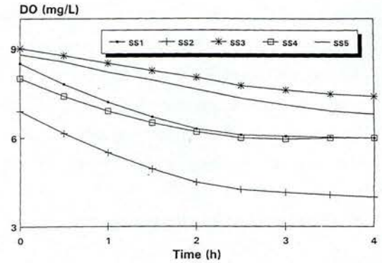
Fig. 4 Effect of temperature on SOD
