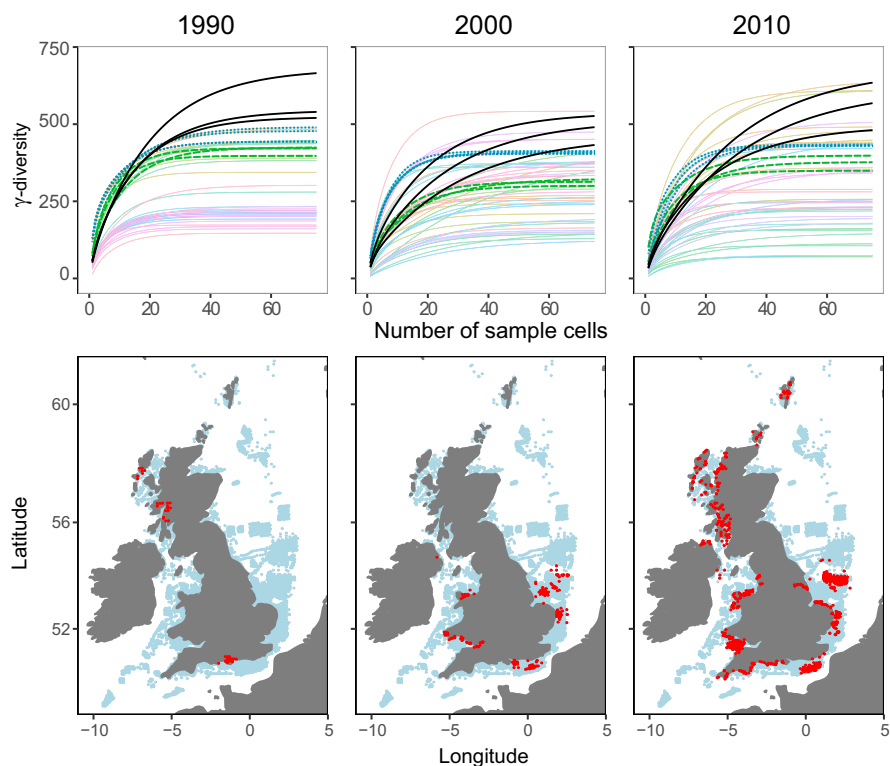
FIGURE 2 Top panels: rarefaction of marine benthic assemblages used to estimate \gamma -diversity for years 1990, 2000 and 2010. Crossing curves demonstrate that the sites rank-order based on richness is not conserved as the number of sample cells (i.e. spatial units) increases, and this feature is consistent over time ( n = 50 cells were randomly selected in 2000 and 2010 where there were data for >50 ). We highlight areas which may have relatively low to intermediate species richness based on a low number of sample cells (black lines) compared with other areas (e.g. blue dotted and green dashed lines) but, because of higher dissimilarity between local assemblages, tend to have some of the highest species richness values at larger scales. Based on these results, we would draw contrasting conclusions about which area was most diverse depending on whether we looked at 1, 20 and 60 sites within a region. Bottom panels: maps show differences in spatial data distribution between respective years (red = data collected in that year, blue = all data)
