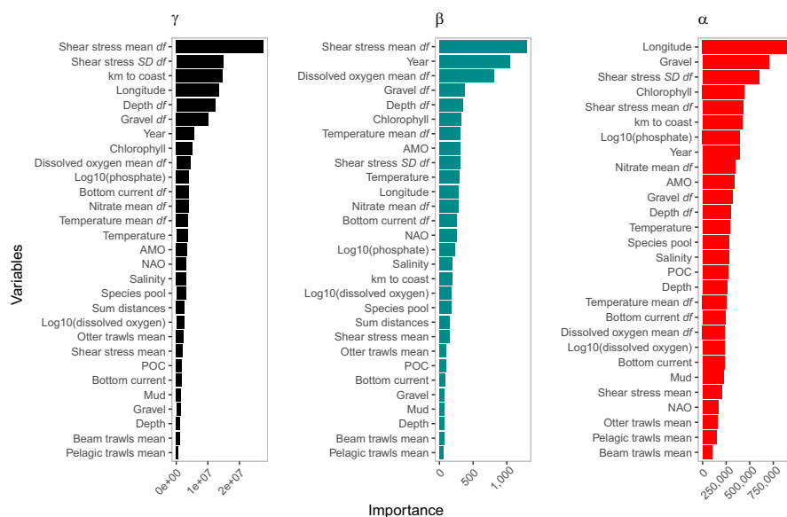
FIGURE 3 Variable importance based on node impurity ordered along the y-axis from most important (top) to least important (bottom) following Random Forest analysis on the combined data. The suffix 'df' represents a variable's heterogeneity based on mean pairwise differences across selected sample cells within a 25 km radius
