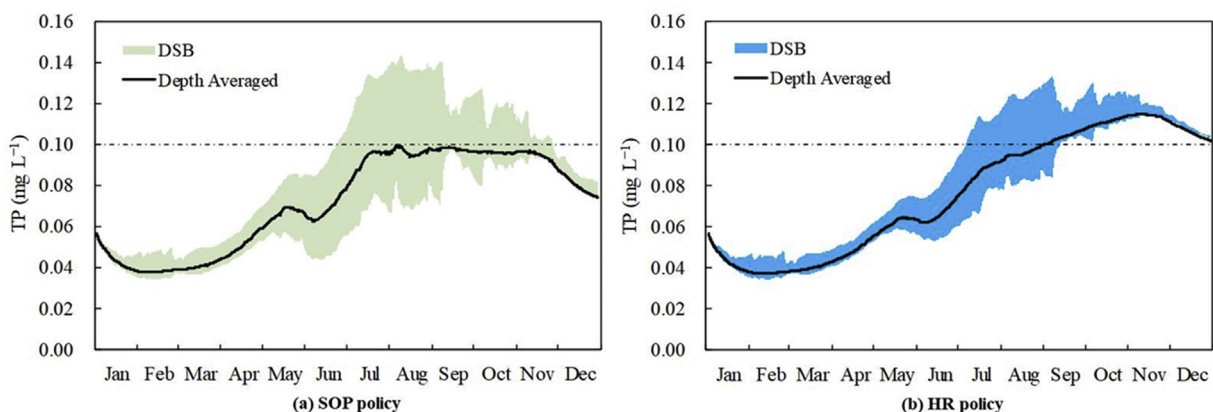
Fig. 4. Plane-averaged TP concentration variations in the reservoir under (a) SOP and (b) HR. DSB represents concentration differences between the surface and bottom layers; the upper boundary shows TP in the bottom layer and the lower boundary shows TP in the surface layer.
