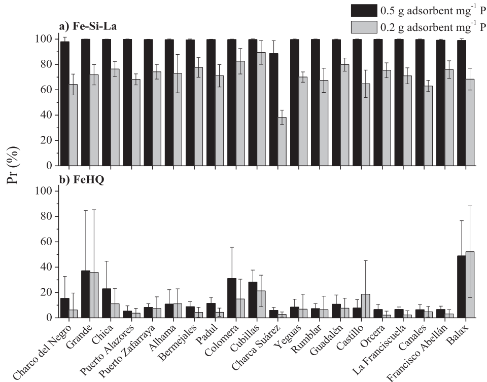
Fig. 5. P removal efficiency (Pr in %) of magnetic adsorbents (Fe-Si-La and FeHQ) for each lake. High adsorbent dosage in black and low in grey. Standard deviation is represented by vertical bars.
