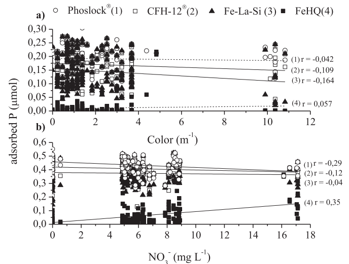
Fig. 3. a) Relation between adsorbed P and color for the four studied adsorbents. b) Relation between adsorbed P and \text{NO}_3^- for the four studied adsorbents. r is the Pearson correlation coefficient. The y-axis values are power-transformed ( x^2 ).
