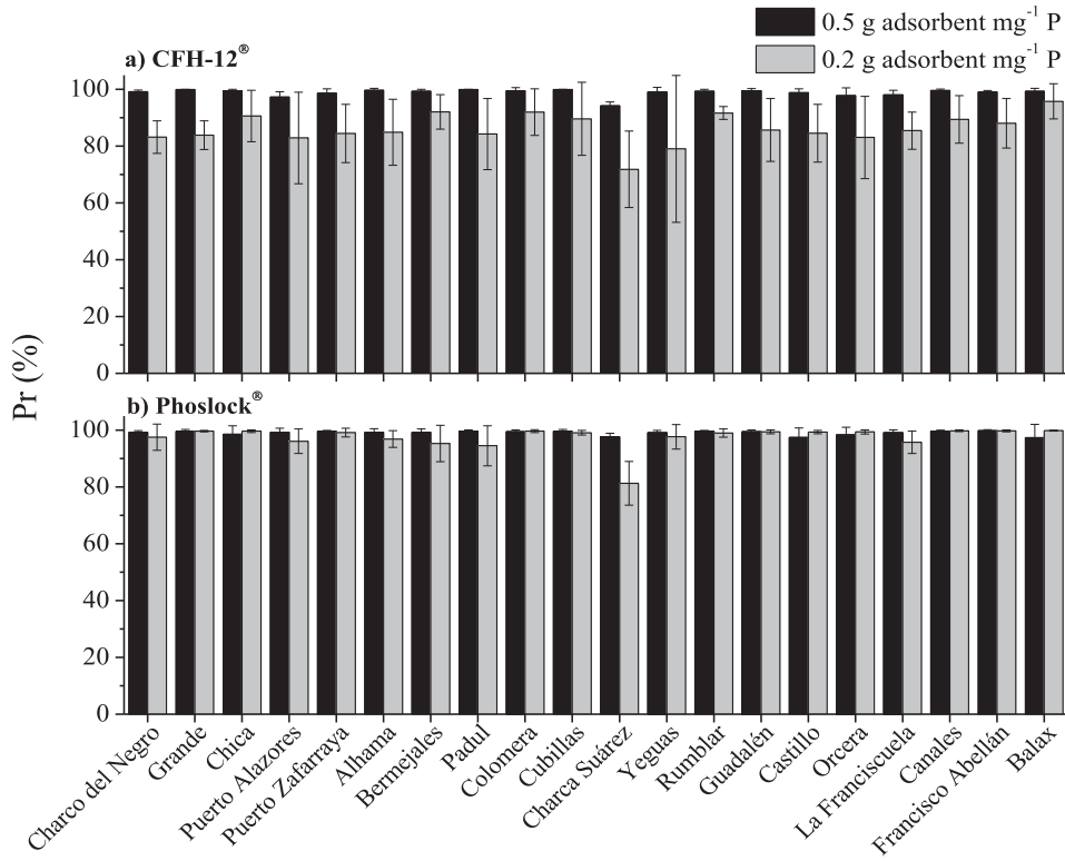
Fig. 4. P removal efficiency (Pr in %) of non magnetic adsorbents (CFH-12 ® and Phoslock ® ) for each lake. High adsorbent dosage in black and low in grey. Standard deviation is represented by vertical bars.
