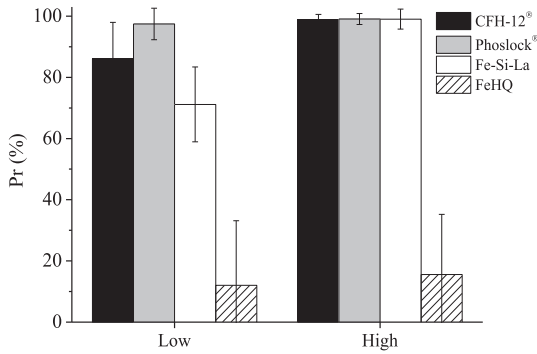
Fig. 2. P removal efficiency (Pr in %) for the merged data of all studied systems as a function of type of adsorbent and adsorbent dosage. Standard deviation is represented by vertical bars.
