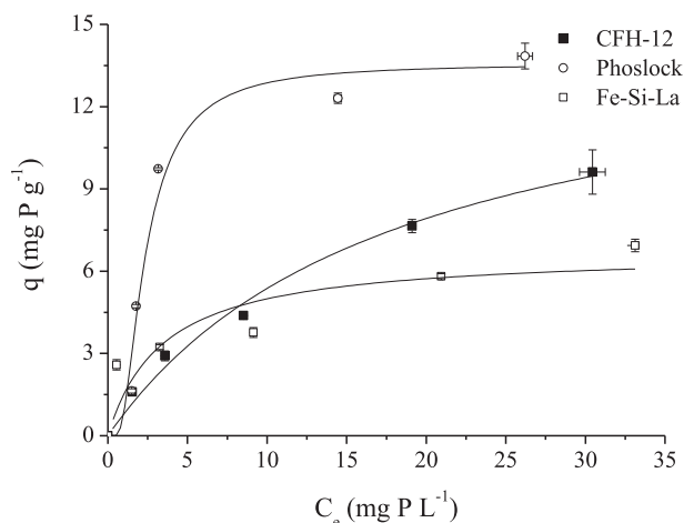
Fig. 1. Adsorption isotherms of CFH-12 ® , Phoslock ® and Fe-Si-La. Adsorbent concentration 1 \text{g L}^{-1} ; pH = 7. Standard deviation is represented by vertical bars.
