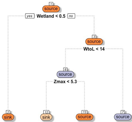
Figure 5. Classification tree model visualizing static predictors of net CO 2 flux, indicated as a net source or sink. WtoL indicates watershed-to-lake area ratio, and Z max indicates maximum lake depth.
