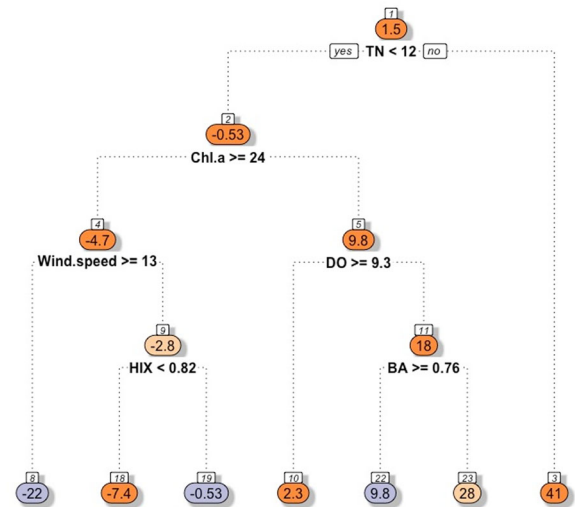
Figure 4. Regression tree model visualizing predictors of discrete \text{CO}_2 flux. Terminal node values represent instantaneous flux rates where influx appears on the left, and efflux on the right. TN indicates total nitrogen ( \text{mg l}^{-1} ), chl. a indicates chlorophyll a ( \mu\text{g l}^{-1} ), DO indicates epilimnetic or surface (integrated 2 m) dissolved oxygen ( \text{mg l}^{-1} ), HIX indicates the humification index, and BA indicates the beta/alpha index.
