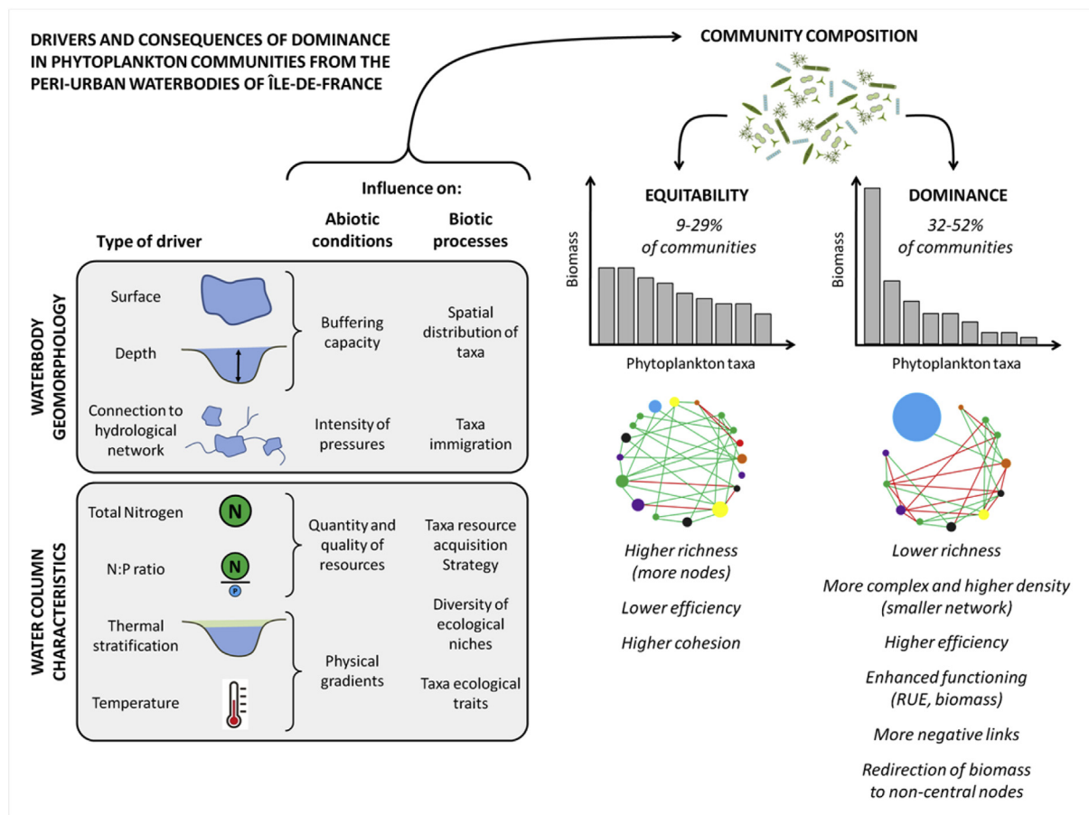
Fig. 3. Drivers and consequences of dominance in phytoplankton communities.
